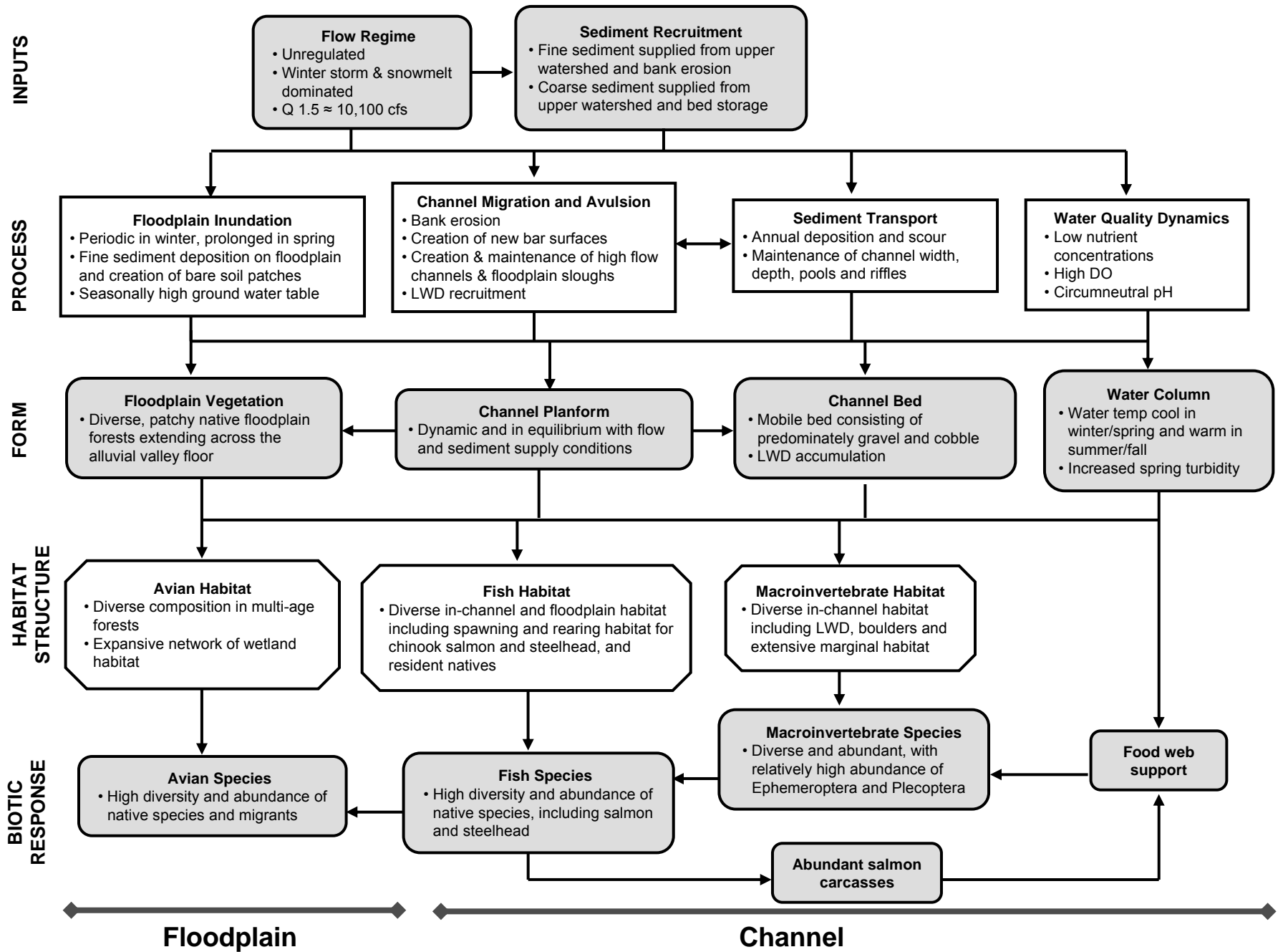
FIGURE 8-1a Conceptual model of reference state processes and linkages in the Merced River Dredger Tailings Reach and at the Merced River Ranch. LWD = large woody debris.
