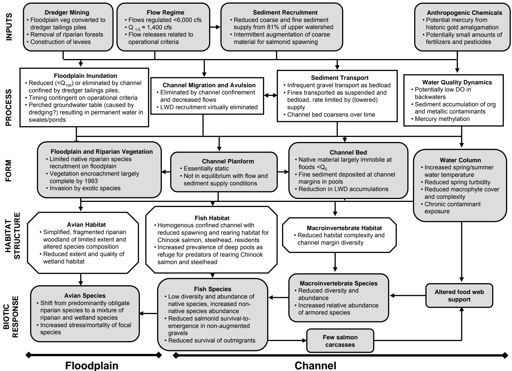
FIGURE 8-1b Conceptual model of current state processes and linkages in the Merced River Dredger Tailings Reach and at the Merced River Ranch.
